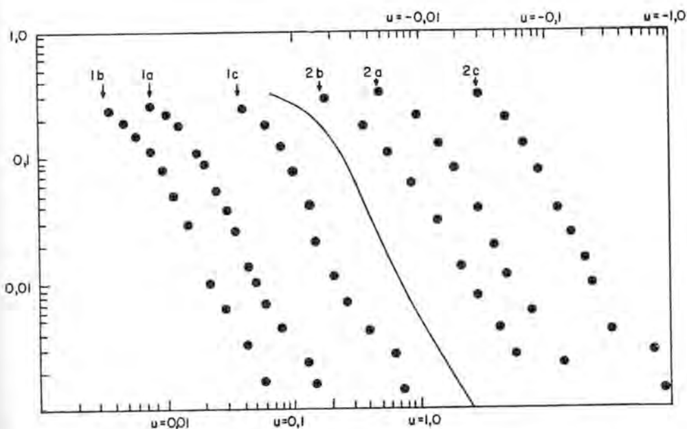
FIGURE E14-5. Composite of doubly logarithmic graphs of positive and negative tails for three kinds of cotton price relatives, together with a plot of the cumulated density function of a stable distribution.
